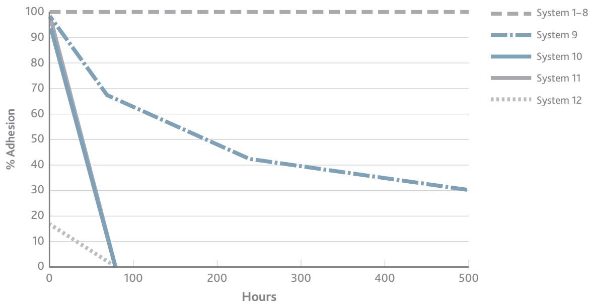
Figure 1. Humidity resistance of CPO primers a,b , % retained adhesion
